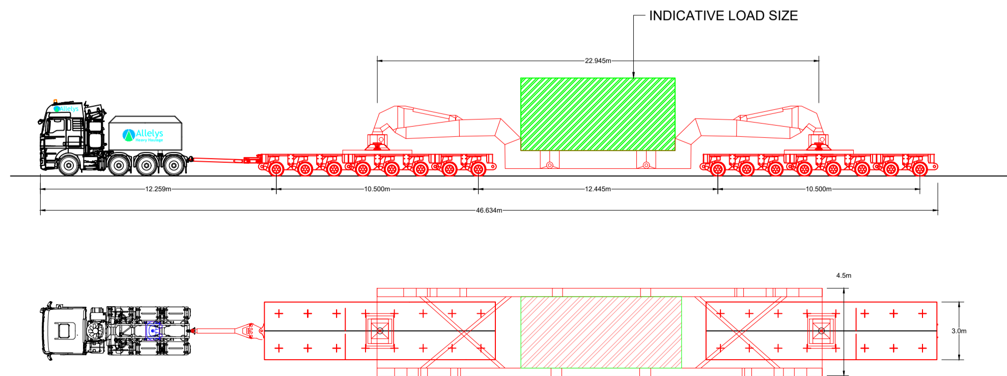
VEHICLE CONFIGURATION - 16-AXLE GIRDER TRAILER
